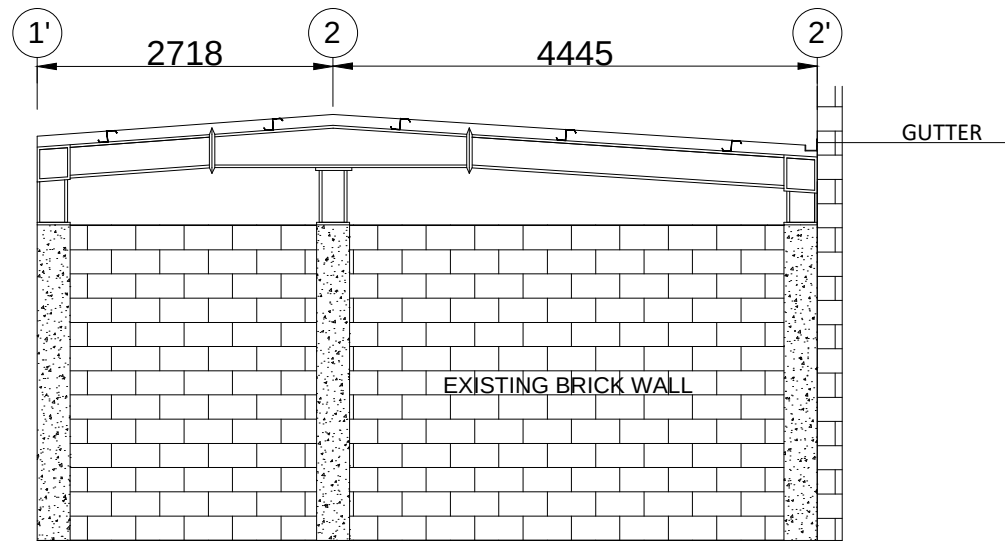
CROSS SECTION GRID-D
